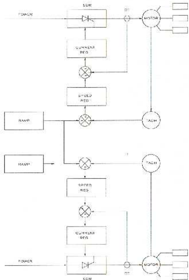
Figure 11 Master/Master Control
