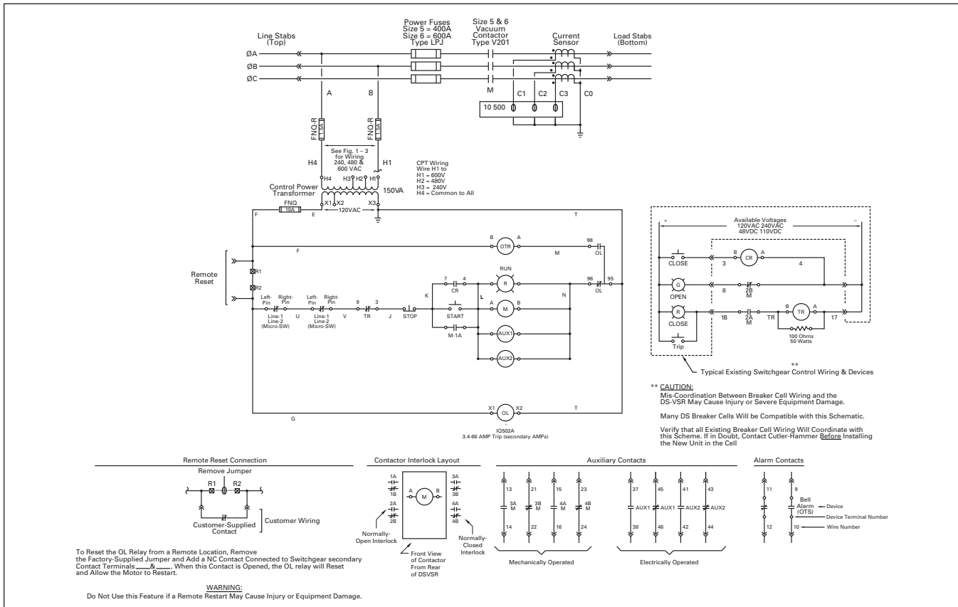
Figure 27-2. DS-VSR-540 Schematic
