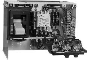
5-Star Replacement Starter Unit (1975 to 1987)
