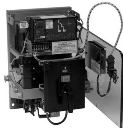
Retrofit Breaker
