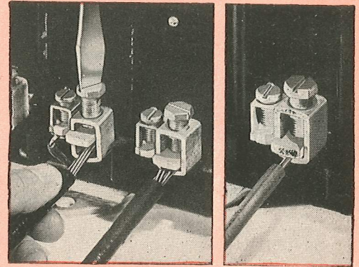
↑ PRESSURE-TYPE CONNECTORS ← STRAIGHT-THROUGH WIRING
